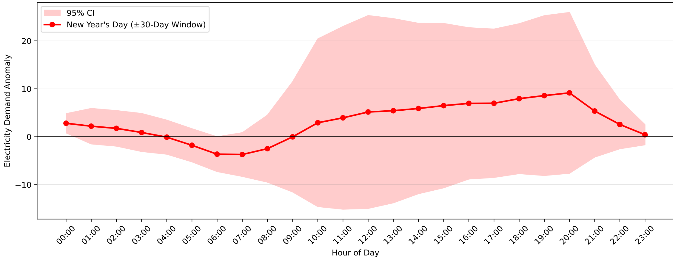
Revesby Demand Anomaly: New Year's Day (2005-2006, \pm 30 -Day Window)
