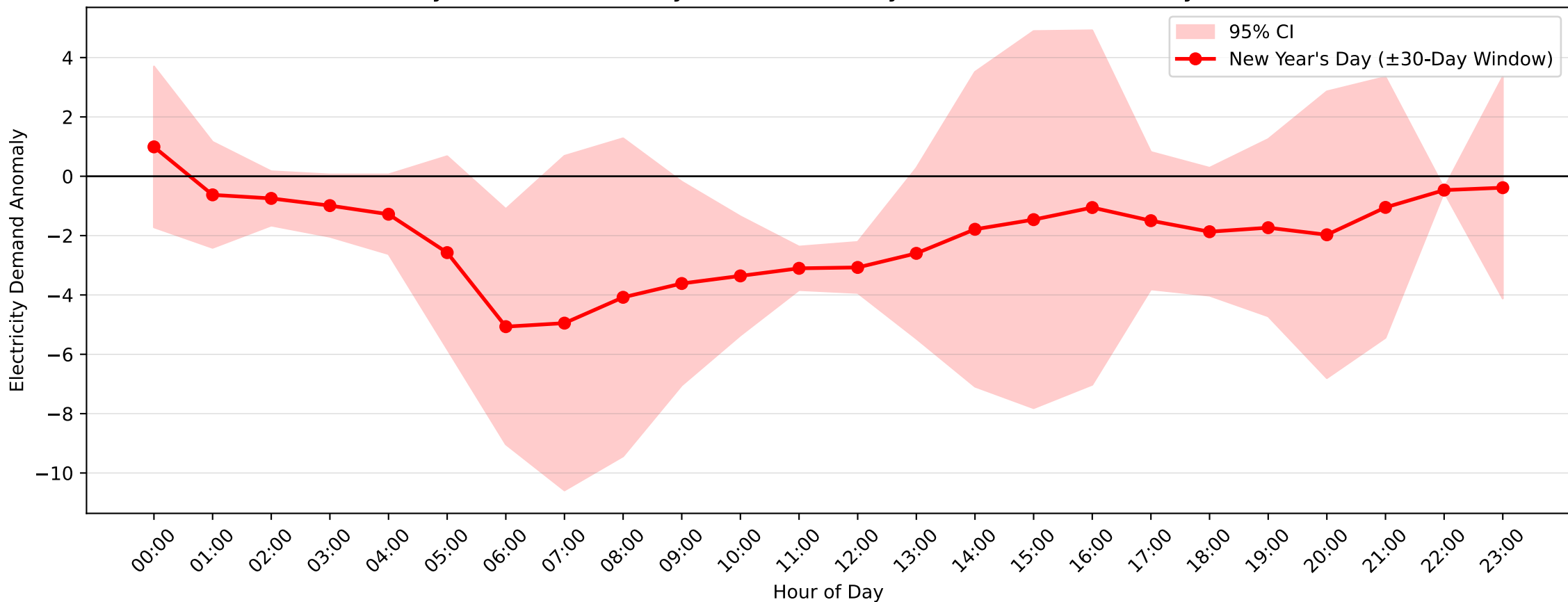
Revesby Demand Anomaly: New Year's Day (2004-2005, \pm 30 -Day Window)
