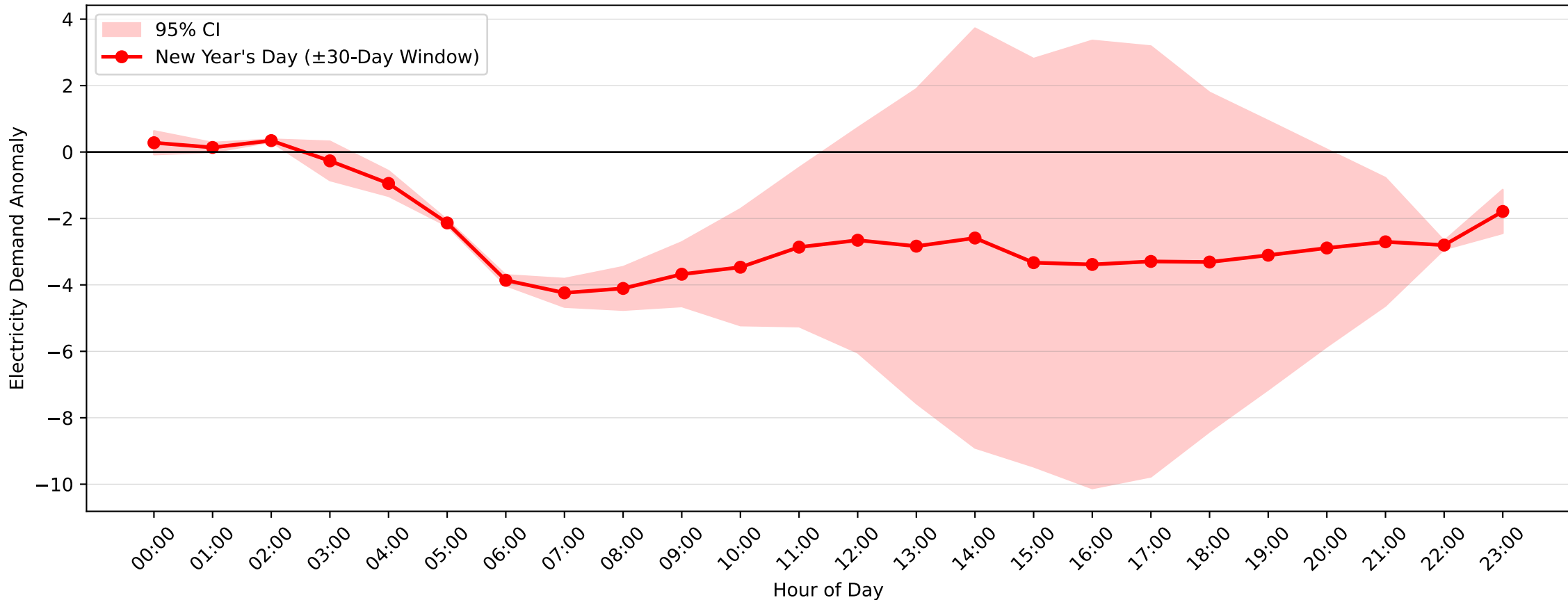
Revesby Demand Anomaly: New Year's Day (2007-2008, \pm 30 -Day Window)
