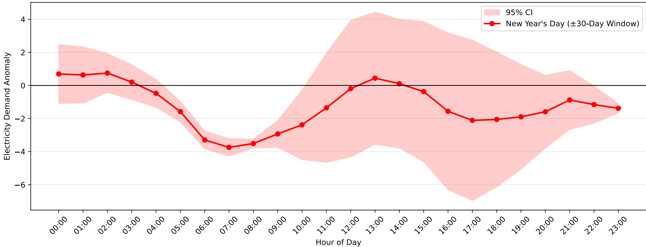
Revesby Demand Anomaly: New Year's Day (2013-2014, \pm 30 -Day Window)
