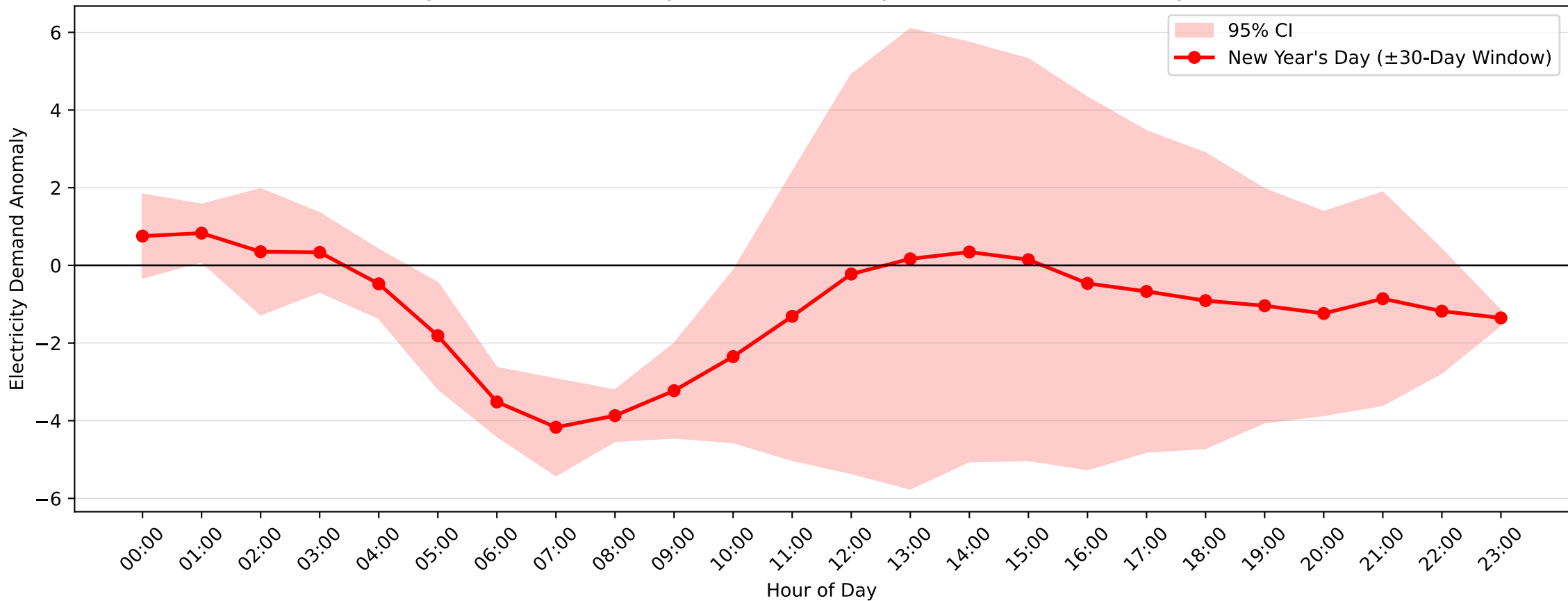
Revesby Demand Anomaly: New Year's Day (2012-2013, \pm 30 -Day Window)
