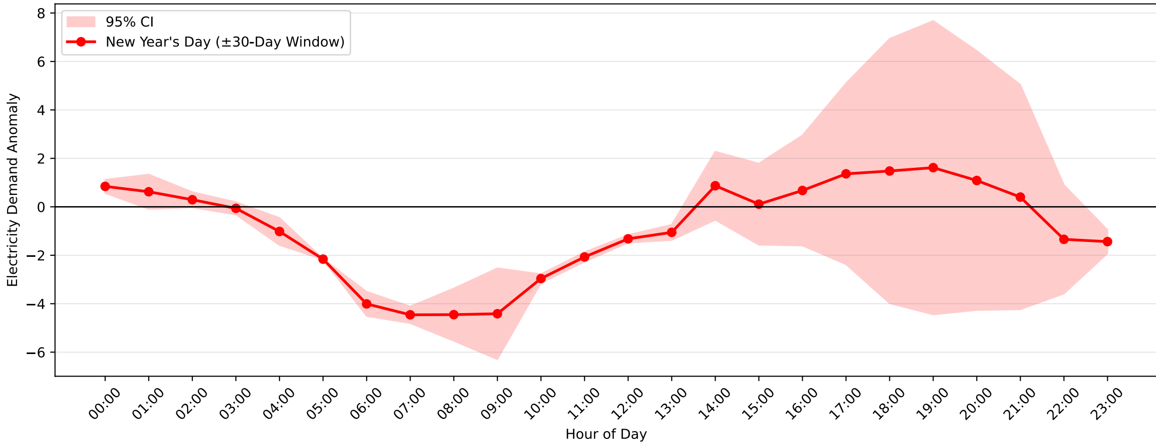
Revesby Demand Anomaly: New Year's Day (2008-2009, \pm 30 -Day Window)
